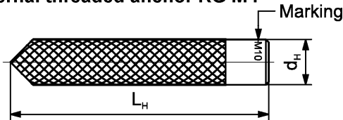
fischer internal threaded anchor RG M I
